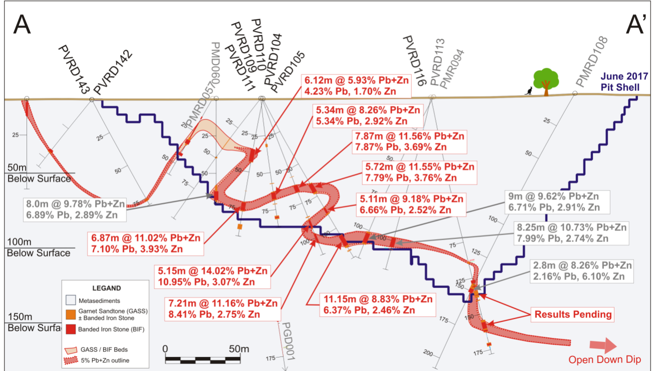
Figure 2. Cross Section through Zones 1, 2 and 3
