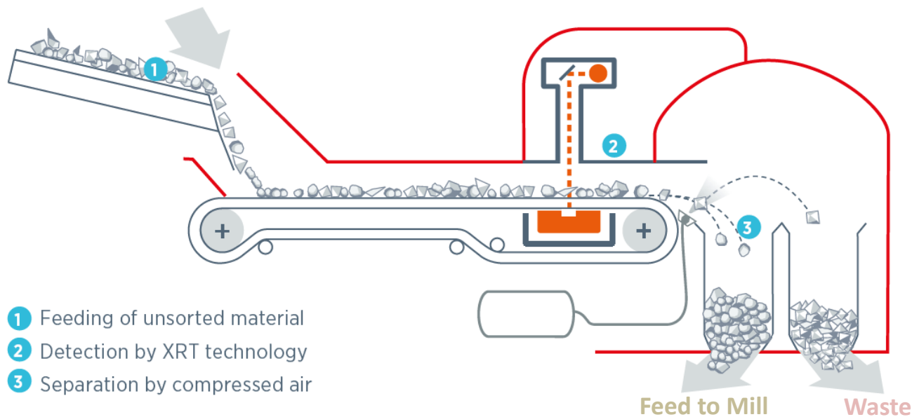
Figure 1. Schematic of the XRT ore sorting process (source: TOMRA)
